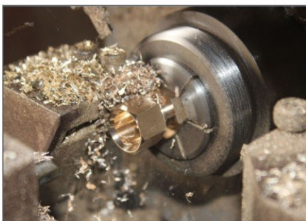
Turning Machine
